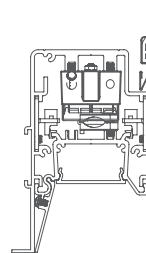
ProTools 60 Linear Perimeter Recessed
