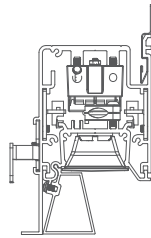
ProTools 60 Linear Wall Graze Recessed
