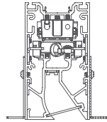
ProTools 60 Linear Wall Wash Recessed
