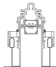
20LRF-RRT Recessed Grid Trim
