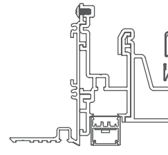
20LPF-SG-RPT Flush Plaster Trim Soft-graze
