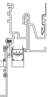
20LPR-SG-RGT Recessed Grid Trim Soft-graze
