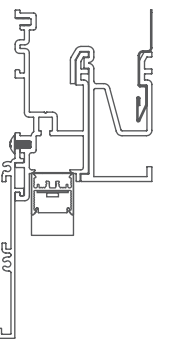
20LPR-SG-RRT Recessed Return Trim Soft-graze
