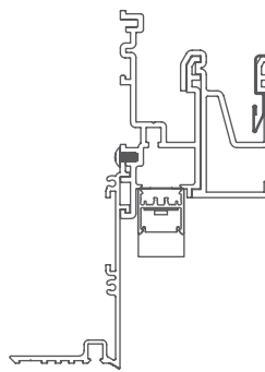
20LPR-SG-RPT Recessed Plaster Trim Soft-graze
