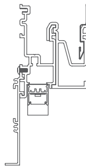
20LPR-SG-RBT Recessed Bezel Trim Soft-graze
