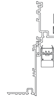
20LPF-RPT Recessed Plaster Trim
