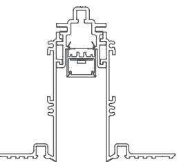
20LRR-RPT Recessed Plaster Trim
