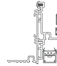
20LPF-RPT Flush Plaster Trim
