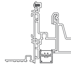
20LPF-SG-RPT Flush Plaster Trim Soft-graze 1·2·5
