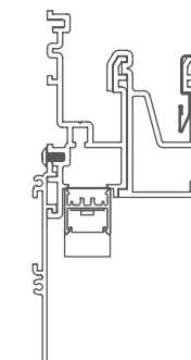
20LPR-SG-RBT Recessed Bezel Trim Soft-graze 1·2·3·4·5
