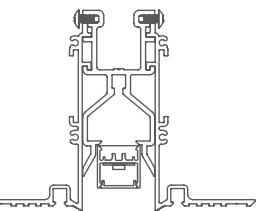
20LRF-RPT Flush Plaster Trim 1·2·3·4·5·6
