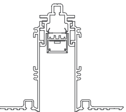
20LRR-RPT Recessed Plaster Trim 1·2·3·4·5
