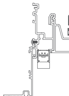
20LPR-SG-RPT Recessed Plaster Trim Soft-graze 1·2·3·4·5
