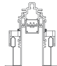
20LRF-RRT Recessed Grid Trim 1·2·3·4·5
