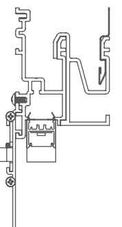
20LPR-SG-RGT Recessed Grid Trim Soft-graze 1·2·3·4·5
