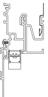
20LPR-SG-RRT Recessed Return Trim Soft-graze 1·2·3·4·5
