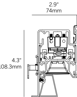
Recessed Louver (RLW, RLB + WG)
