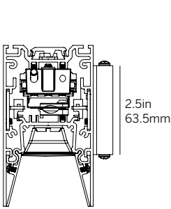
Recessed Louver (RLW, RLB)
