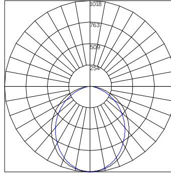
ILLUMINANCE - 24" ROL-105 P4 3000K WG-60PTL-...-S-24-930-ROL-105-P4-...-W-W*
