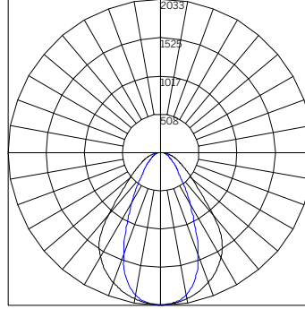
ILLUMINANCE - 24" RML-80 P4 3000K WG-60PTL-...-S-24-930-RML-80-P4-...-W-W*
