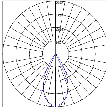
ILLUMINANCE - 24" RLW-50 P4 3000K WG-60PTL-...-S-24-930-RLW-50-P4-...-W-W*
