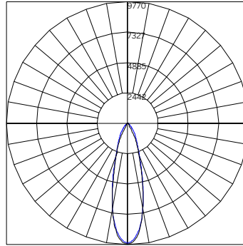
ILLUMINANCE - 24" RLW-35 P4 3000K WG-60PTL-...-S-24-930-RLW-35-P4-...-W-W*
