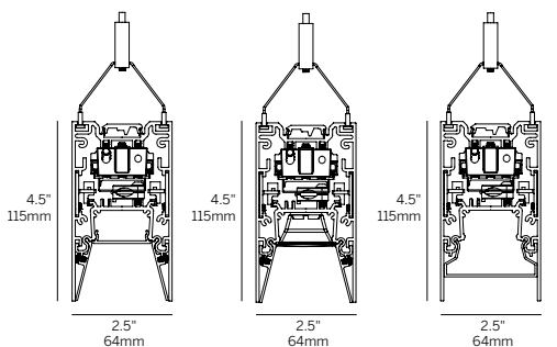
Recessed Micro-prismatic Lens (RML)
