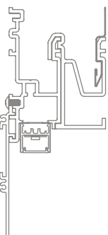
20 Linear Perimeter Regressed Return Trim Soft-graze
