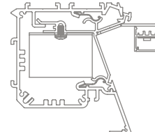
20 Z Cove Fixed Vertical
