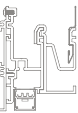
20 Linear Perimeter Flush Return Trim Soft-graze
