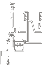
20 Linear Perimeter Regressed Grid Trim Soft-graze
