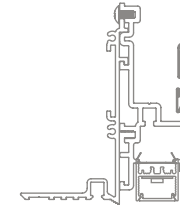
20 Linear Perimeter Flush Plaster Trim
