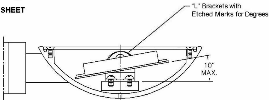
Detail - LED Rotation Half Scale
