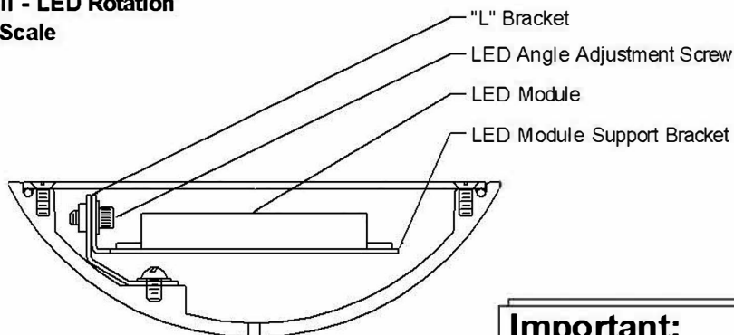
Detail - LED Rotation, 90° View Half Scale
