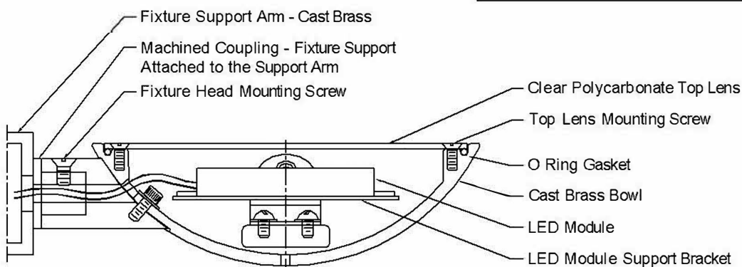
Detail - Cross Section - Support Bracket Half Scale
