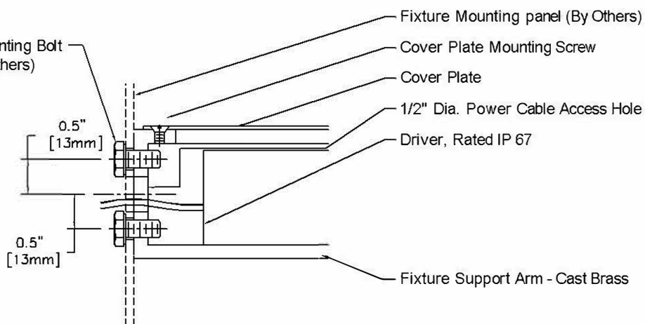
Detail - Cross Section - Fixture Support Arm Half Scale
