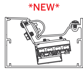
*NEW* Box Cove 2 Surface/Mullion Mount
