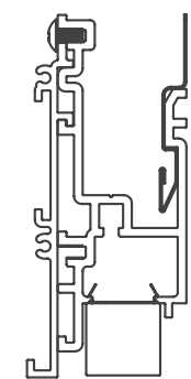
20 Linear Perimeter Flush Lens Return Trim
