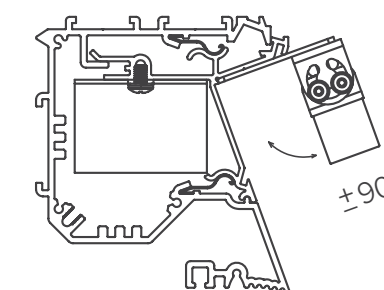
20 Z Cove Adjustable Graze Plaster Trim
