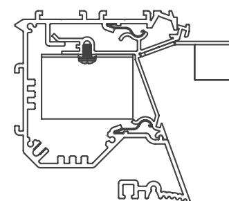
20 Z Cove Graze Plaster Trim
