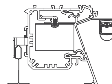
20 Z Cove Graze Grid Trim
