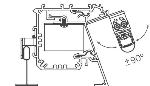
20 Z Cove Adjustable Graze Grid Trim
