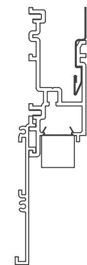
20 Linear Perimeter Regressed Lens Return Trim
