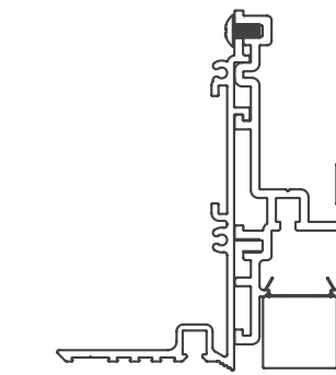
20 Linear Perimeter Flush Lens Plaster Trim
