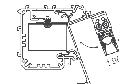
20 Z Cove Adjustable Graze Bezel Trim
