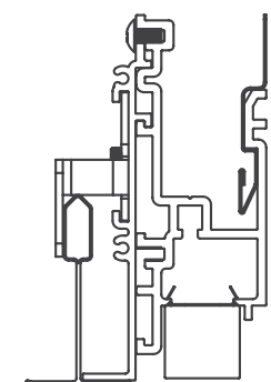
20 Linear Perimeter Flush Lens Grid Trim
