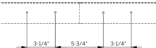
Figure 4: Wall Reference for Holes
