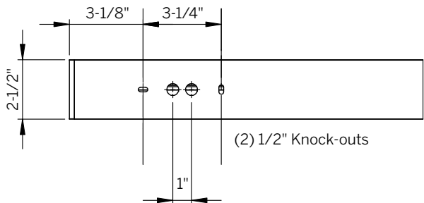
Figure 2: Rear View of Fixture
