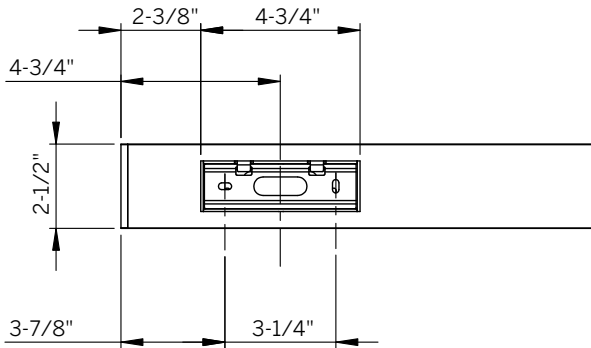
Figure 2: Rear View of Fixture
