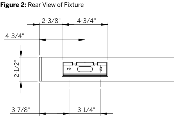
Figure 2: Rear View of Fixture
