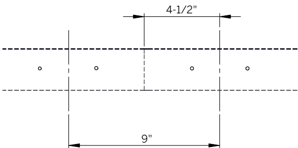
Figure 2: Rear View of Fixture
