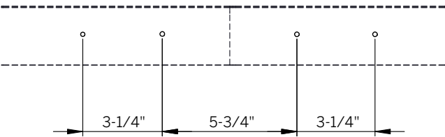
Figure 4: Wall Reference for Holes
