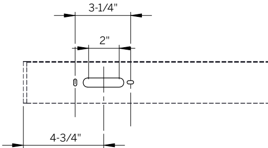
Figure 4: Wall Reference for Holes
