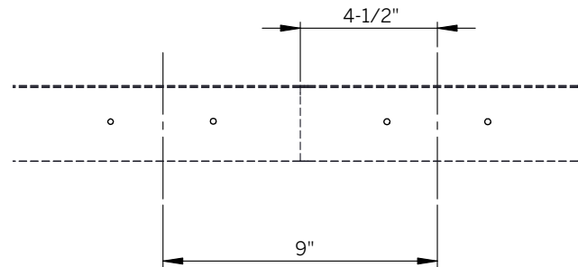
Figure 2: Rear View of Fixture
