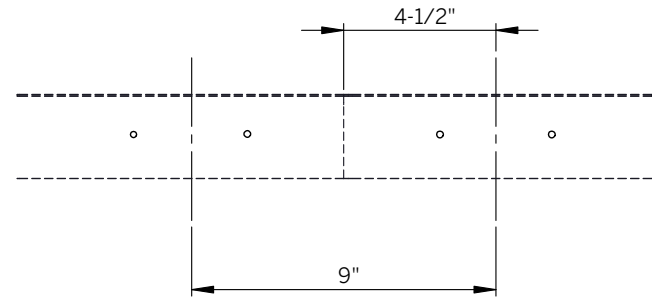
Figure 2: Rear View of Fixture
