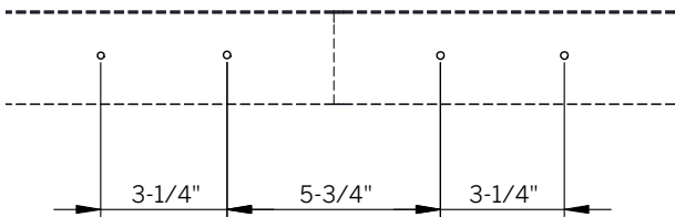
Figure 4: Wall Reference for Holes
