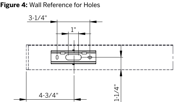
Figure 4: Wall Reference for Holes
