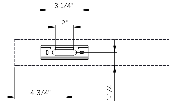
Figure 4: Wall Reference for Holes
