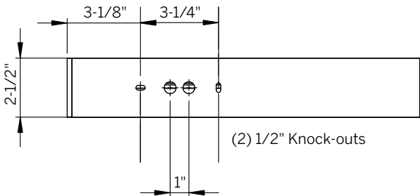
Figure 2: Rear View of Fixture
