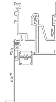
20 Linear Perimeter Regressed Bezel Trim Soft-graze
