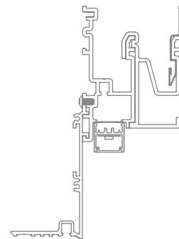
20 Linear Perimeter Regressed Plaster Trim Soft-graze
