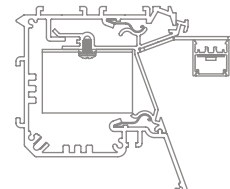
20 Z Cove Fixed Vertical
