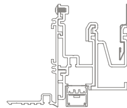
20 Linear Perimeter Flush Plaster Trim Soft-graze
