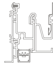
20 Linear Perimeter Flush Bezel Trim Soft-graze
