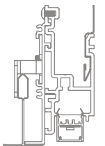
20 Linear Perimeter Flush Grid Trim
