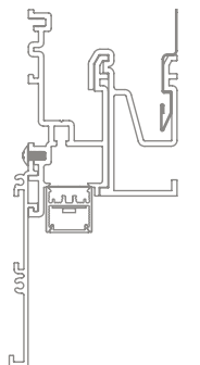
20 Linear Perimeter Regressed Return Trim Soft-graze
