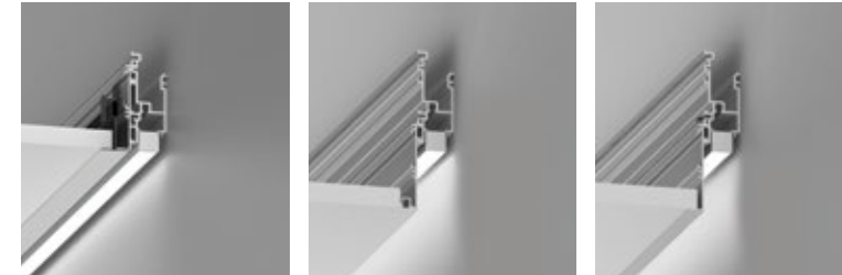
20 Linear Perimeter Flush Grid Trim 20LPF-RGT 20 Linear Perimeter Regressed Plaster Trim 20LPR-RPT 20 Linear Perimeter Regressed Bezel Trim 20LPR-RBT
