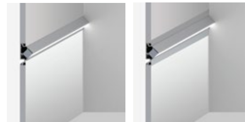
20 Linear Semi-Recessed Floor Wash Plaster Trim WG 20LCFW-SRPT 20 Linear Semi-Recessed Floor Wash Bezel Trim 20LCFW-SRBT
