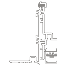
20 Linear Perimeter Flush Plaster Trim
