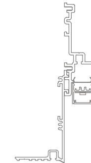
20 Linear Perimeter Regressed Plaster Trim
