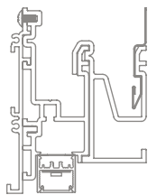
20 Linear Perimeter Flush Return Trim Soft-graze
