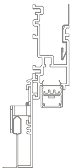
20 Linear Perimeter Regressed Grid Trim
