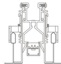
20 Linear Flush Grid Trim
