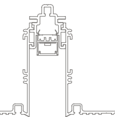
20 Linear Regressed Plaster Trim
