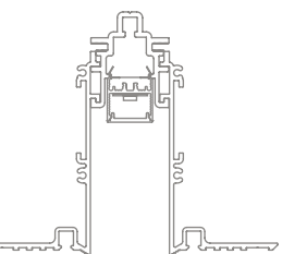
20 Linear Regressed Plaster Trim
