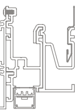
20 Linear Perimeter Flush Return Trim Soft-graze
