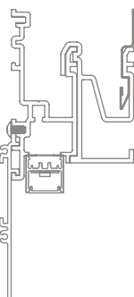
20 Linear Perimeter Regressed Return Trim Soft-graze
