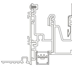
20 Linear Perimeter Flush Plaster Trim Soft-graze
