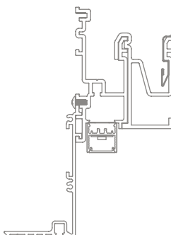
20 Linear Perimeter Regressed Plaster Trim Soft-graze
