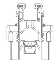
20 Linear Flush Grid Trim
