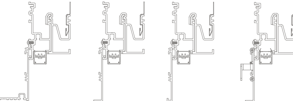
20 Linear Perimeter Regressed Plaster Trim Soft-graze 20 Linear Perimeter Regressed Bezel Trim Soft-graze 20 Linear Perimeter Regressed Return Trim Soft-graze 20 Linear Perimeter Regressed Grid Trim Soft-graze
