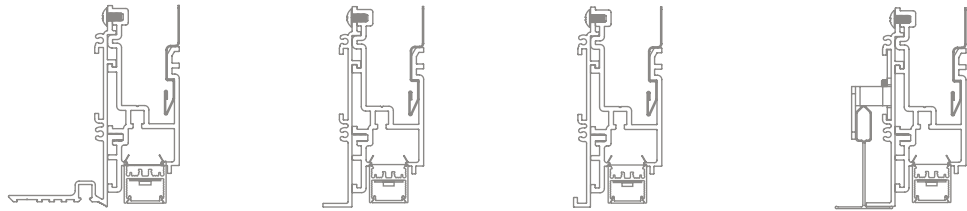
20 Linear Perimeter Flush Plaster Trim 20 Linear Perimeter Flush Bezel Trim 20 Linear Perimeter Flush Return Trim 20 Linear Perimeter Flush Grid Trim
