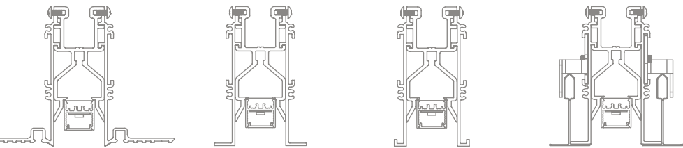
20 Linear Flush Plaster Trim 20 Linear Flush Bezel Trim 20 Linear Flush Return Trim 20 Linear Flush Grid Trim
