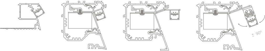
20 Mini Z Cove 20 Z Cove Fixed 20 Z Cove Fixed Vertical 20 Z Cove Adjustable
