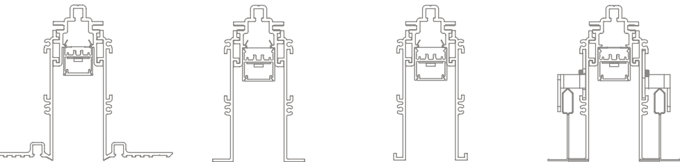
20 Linear Regressed Plaster Trim 20 Linear Regressed Bezel Trim 20 Linear Regressed Return Trim 20 Linear Regressed Grid Trim
