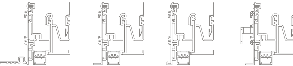
20 Linear Perimeter Flush Plaster Trim Soft-graze 20 Linear Perimeter Flush Bezel Trim Soft-graze 20 Linear Perimeter Flush Return Trim Soft-graze 20 Linear Perimeter Flush Grid Trim Soft-graze
