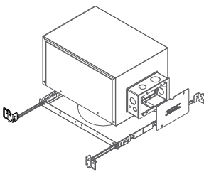
Insulated Ceiling Housing (IC) Chicago Plenum Housing (CP)
