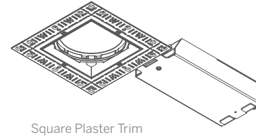
Square Plaster Trim Housing
