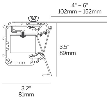
Bezel Trim (RBT) with optional in-fill panel
