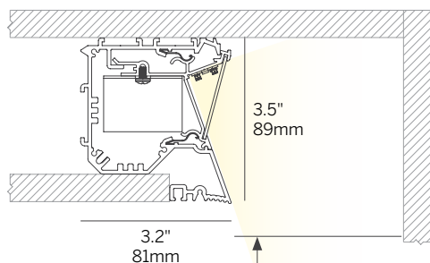
Plaster Trim (RPT)
