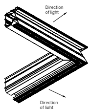
Inside Corner (PI)
