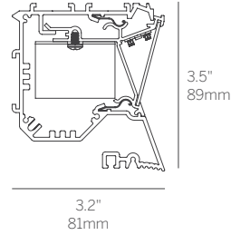
Plaster Trim (RPT)
