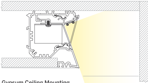
Gypsum Ceiling Mounting
