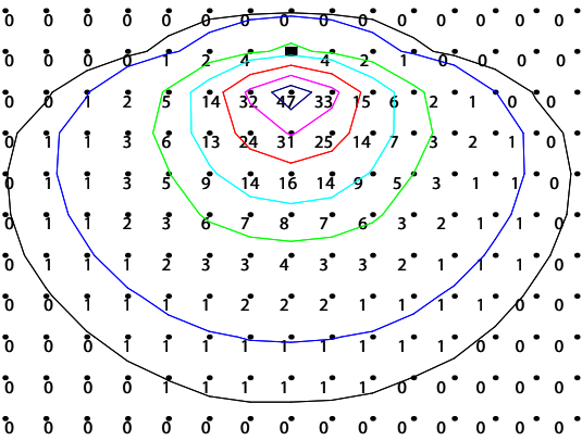
ISOILLUMINANCE DIAGRAM - 11W 3000K Asymmetric 1 PEA-LBOGR-AE-30-11-ID-30-AS
