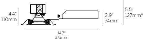
Recessed Plaster Trim (RPT)
