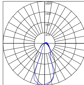
ILLUMINANCE - 48" LL45W H 3500K WG-20LPR-...-S-48-H-935-...-LL45W-W 1
