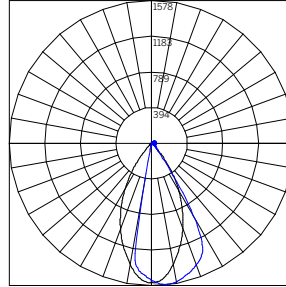
ILLUMINANCE - 48" LL45B H 3500K WG-20LPR-...-S-48-H-935-...-LL45B-W 1
