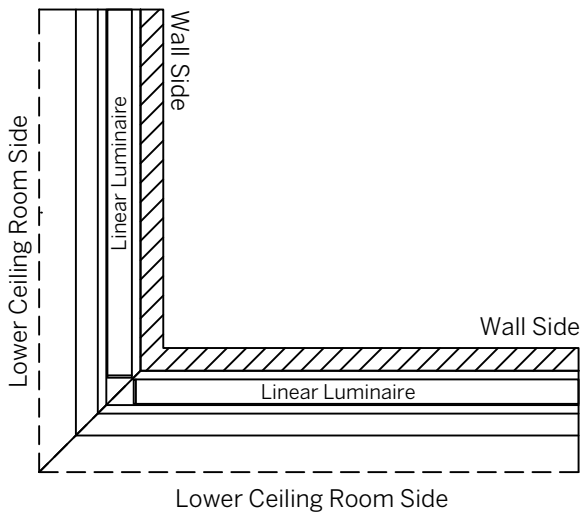
OUTSIDE CORNER (PO)
