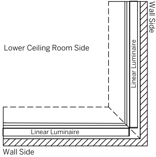
INSIDE CORNER (PI)
