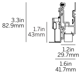
Recessed Grid Trim (RGT9/RGT15)
