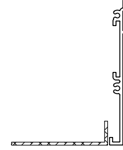
Return Trim
