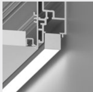
high-efficiency lens
