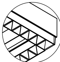
Mitered / Welded Haousing Butted Lens (LL45)
