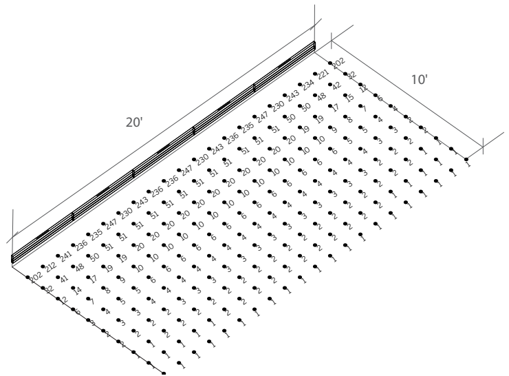
ISOILLUMINANCE - 48" GE 6.5W/FT 3000K LL-DIR-LPMGR-S-RUN-65-X-30-GE*
