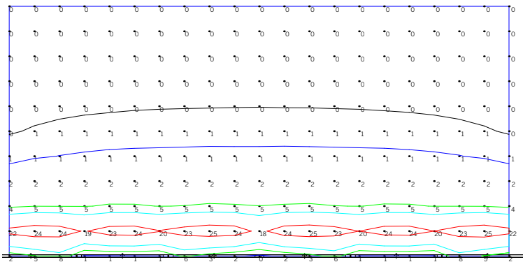
ISOILLUMINANCE DIAGRAM - 4W 3000K General Illumination Continuous Run 1 DIR-LPMGR-S-RUN-4-X-30-GE
