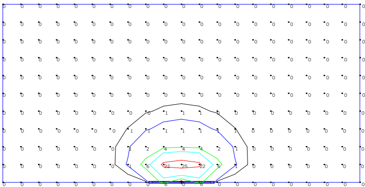
ISOILLUMINANCE DIAGRAM - 4W 3000K General Illumination Single Fixture 1 DIR-LPMGR-S-40-4-X-30-GE
