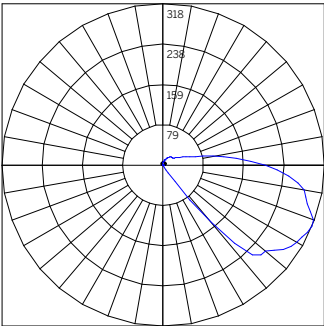
ISOILLUMINANCE DIAGRAM - 4W 3000K General Illumination Continuous Run 1 DIR-LPMGR-S-RUN-4-X-30-GE
