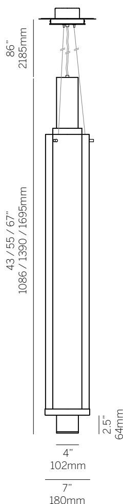
Cylinder downlight
