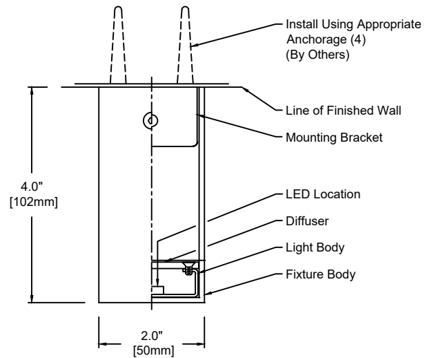
Plan / Cross Section
