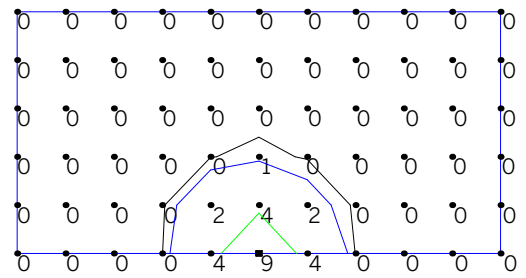
ISOILLUMINANCE DIAGRAM - 1W 3000K Asymmetric 1 EN66-SWH-ME-16-1-CC-30-AS 2
