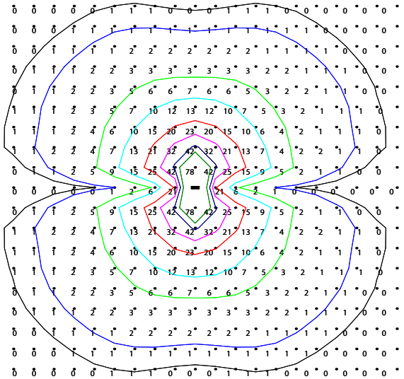
ISOILLUMINANCE DIAGRAM - 20W 3000K General Illumination¹ RYO-BOGR-RE-44-20-ID-30-GE
