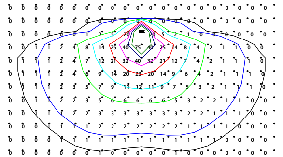
ISOILLUMINANCE DIAGRAM - 20W 3000K General Illumination¹ RYO-BOGR-AE-44-20-ID-30-GE
