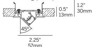
Grid Ceiling (SRGT9/SRGT15)
