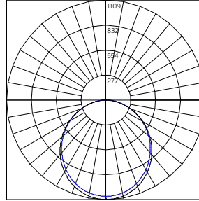
ILLUMINANCE - 48" OD H 3500K WG-20LD-...-S-48-H-935-...-OD-X-XXX-X-XX-W 1
