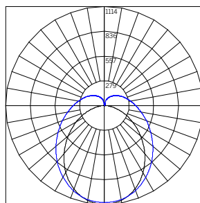
BEAM ANGLE (0-180) = 130.1 BEAM ANGLE (90-270) = 97.2
