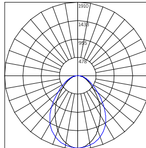
ILLUMINANCE - 48" MPL H 3500K WG-20LD-...-S-48-H-935-...-MPL-X-XXX-X-XX-W 1
