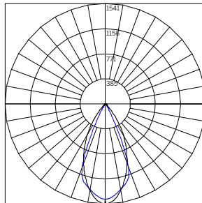
BEAM ANGLE (0-180) = 45.3 BEAM ANGLE (90-270) = 49.7
