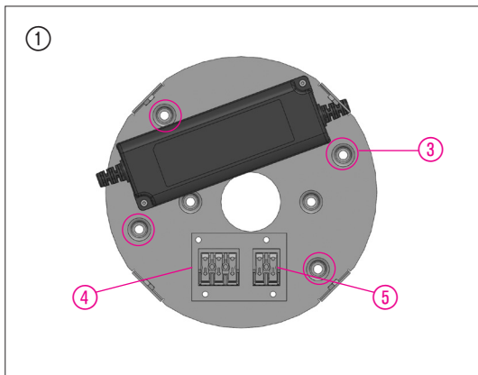
CEILING 2: Baldachin DBSA 200 ( Ø 206 mm )
