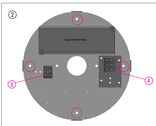
CEILING 4: Baldachin DBSA 250( Ø 250 mm )
