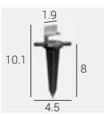
83351 Spike with bracket (requires linear profile or clip ordered separately)
