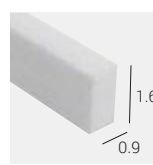
*99521 Polystyrene Concrete-pour preparation kit for 83034 / C-K100009 profiles only (not to be used on curved runs) 1.6"H x 0.9"W x 39.8"L
