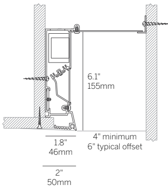
Gypsum Ceiling Mounting Plaster Trim (RPT)
