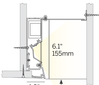
Plaster Trim (RPT)
