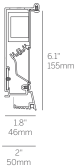
Plaster Trim (RPT)
