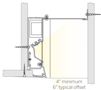
Gypsum Ceiling Mounting (shown with optional infill panel)
