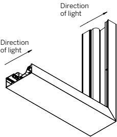
Plane To Plane Inside Corner (PPI)
