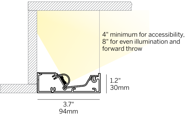
Snap On Satin Diffuser (SSD)
