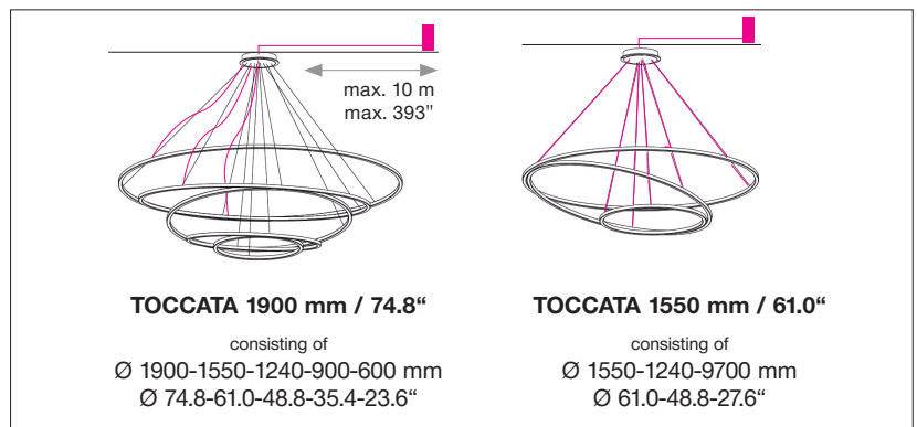
TOCCATA 1900, Mounting version ①
