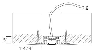
cut-out dimensions 1.5" wide X length + 1/4"
