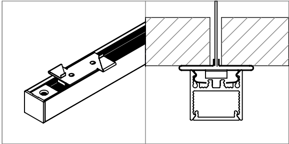
Square Lay-In Grid Clip (GT15)
