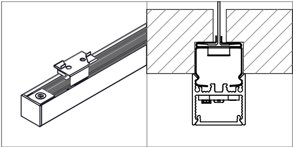
Tegular Grid Clip (GT9T)
