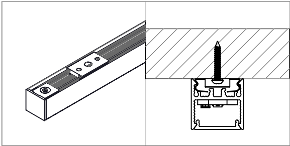
Screw Clip (SC)
