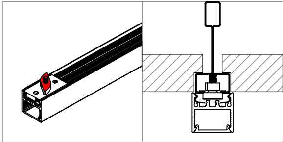
9/16" BOLT SLOT TEGULAR CLIP (1/4" REVEAL) (BS9T)
