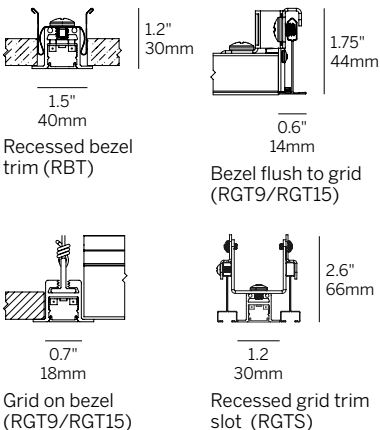
Mounting options
