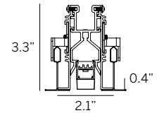
Recessed Grid Trim (RGT9/RGT15)
