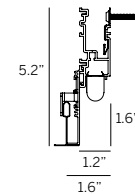
Recessed Grid Trim (RGT9/RGT15)
