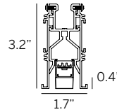
Recessed Return Trim (RRT)
