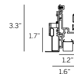
Recessed Grid Trim (RGT9/RGT15)
