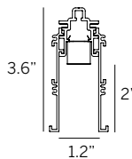
Recessed Return Trim (RRT)
