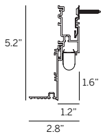
Recessed Plaster Trim (RPT)
