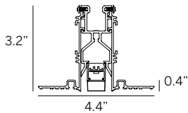
Recessed Plaster Trim (RPT)
