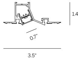
4. 20 Linear Wall Wash Recessed Plaster Trim - Satin Opal Lens WG-20LWW-RPT
