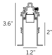
Recessed Bezel Trim (RBT) (shown)
