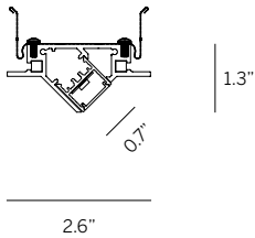
1. 20 Linear Semi Recessed Wall Wash Recessed Plaster Trim - Satin Opal Lens WG-20LWW-SRPT-OD
