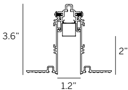
Recessed Plaster Trim (RPT)
