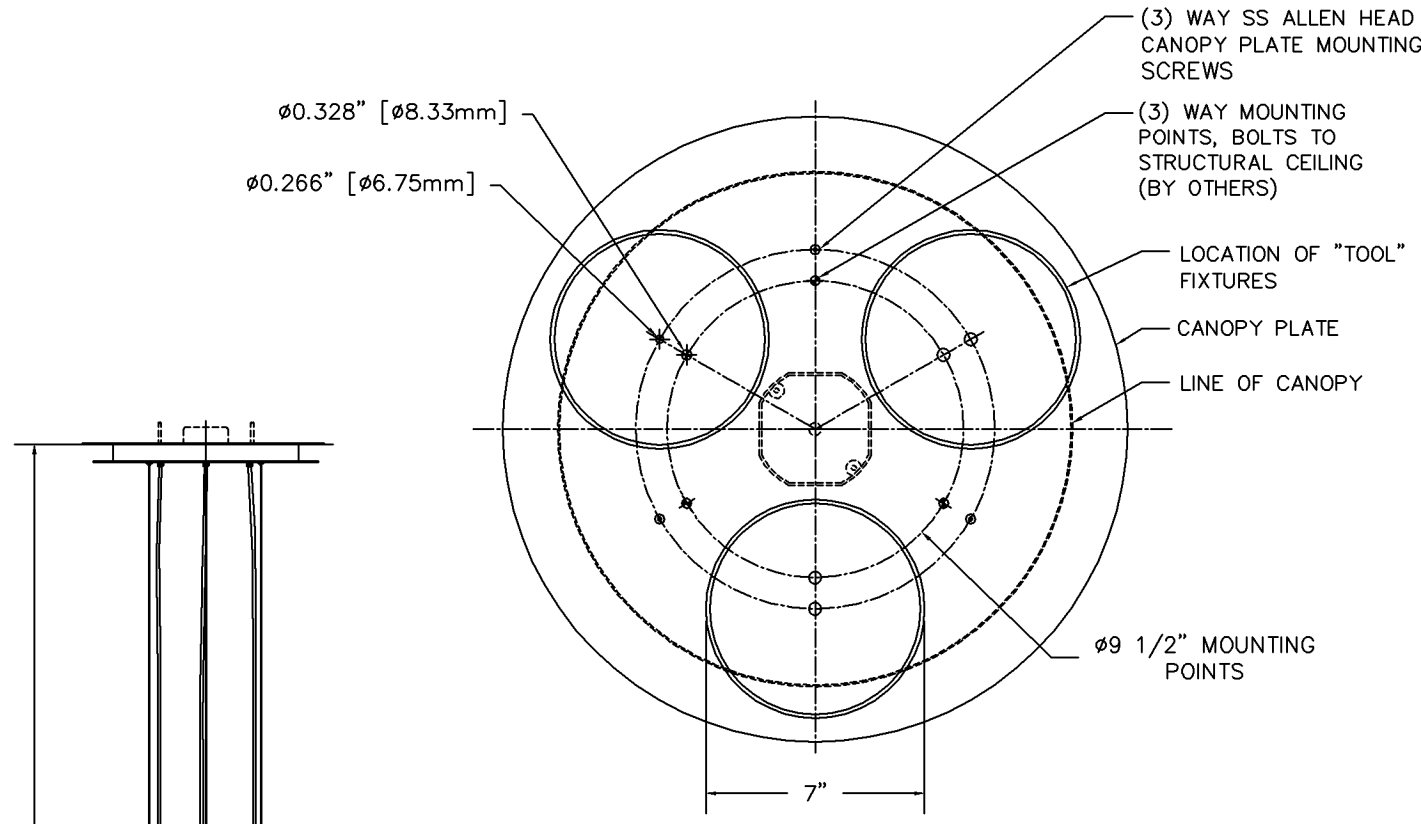
REFLECTED PLAN SCALE : NTS
